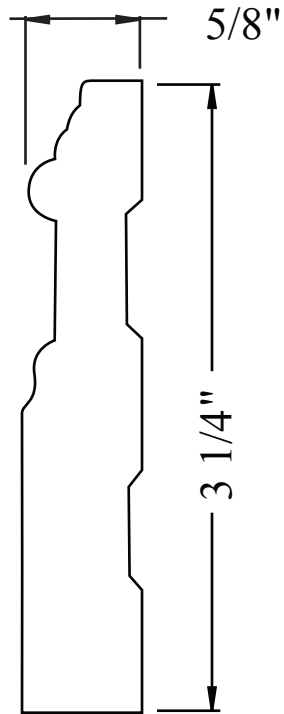
PL305-15CA 5/8" x 3 1/4" FULL SCALE
