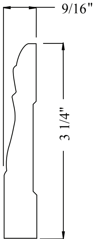
PL366-14BA 9/16" x 3 1/4" FULL SCALE
