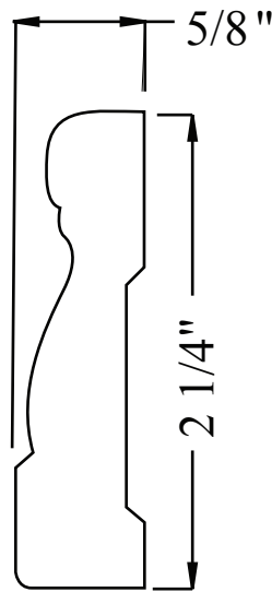
PL313-15CA 5/8" x 2 1/4" FULL SCALE
