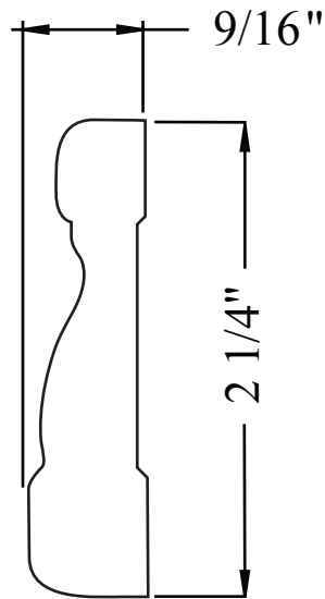
PL314-14CA 9/16" x 2 1/4" FULL SCALE
