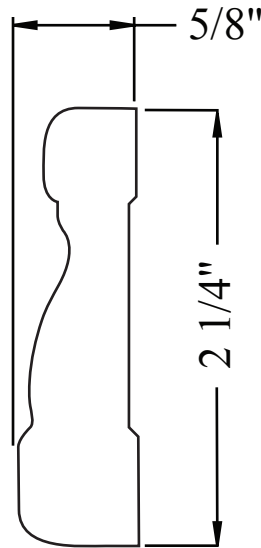
PL314-15CA 5/8 " x 2 1/4" FULL SCALE
