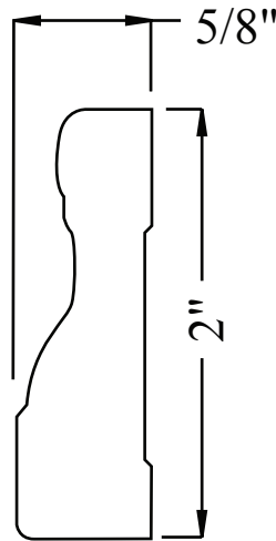
PL677-15CA 5/8" x 2" FULL SCALE
