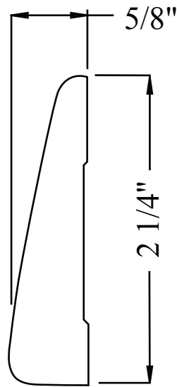
PL106-15CA 5/8" x 2 1/4" FULL SCALE
