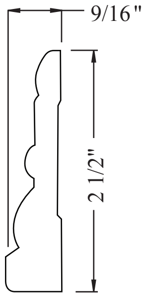
PL211-14CA 9/16" x 2 1/2" FULL SCALE
