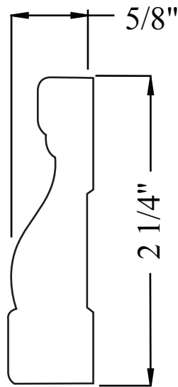
PL311-15CA 5/8" x 2 1/4" FULL SCALE
