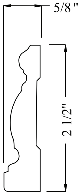
PL322-15CA 5/8" x 2 1/2" FULL SCALE
