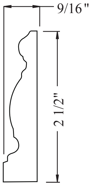
PL323-14CA 9/16" x 2 1/2" FULL SCALE
