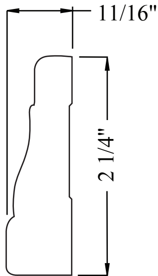
PL357-17CA 11/16" x 2\ 1/4" FULL SCALE
